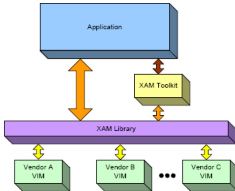
Figure 1. XAM software architecture.
