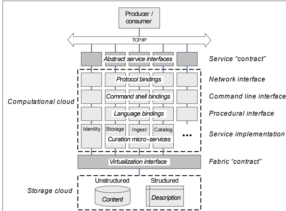
Figure 2. Micro-service stack.
